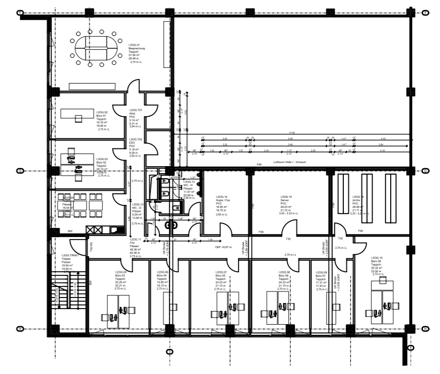
layout office (2nd floor)
